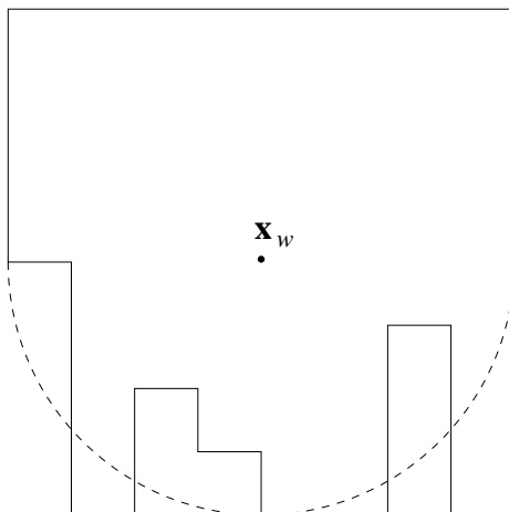
Figure 1: Set S within the square I_w \times [0, 2^{-2n}] .
